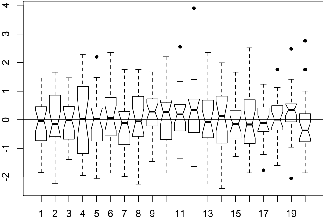
Notched boxplots of N(0,1) for n=25
